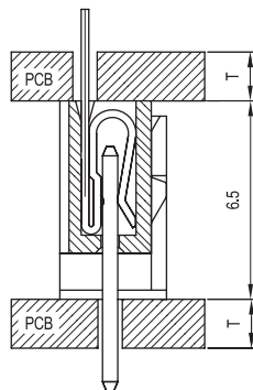
PCB ASSY
